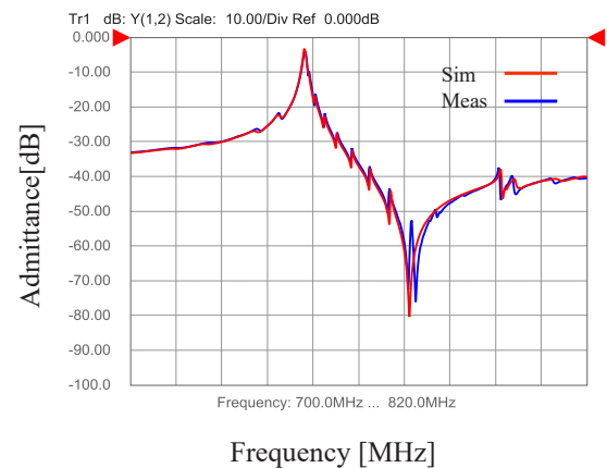
Figure 3 Measured and simulated admittance of 1-Port resonator
